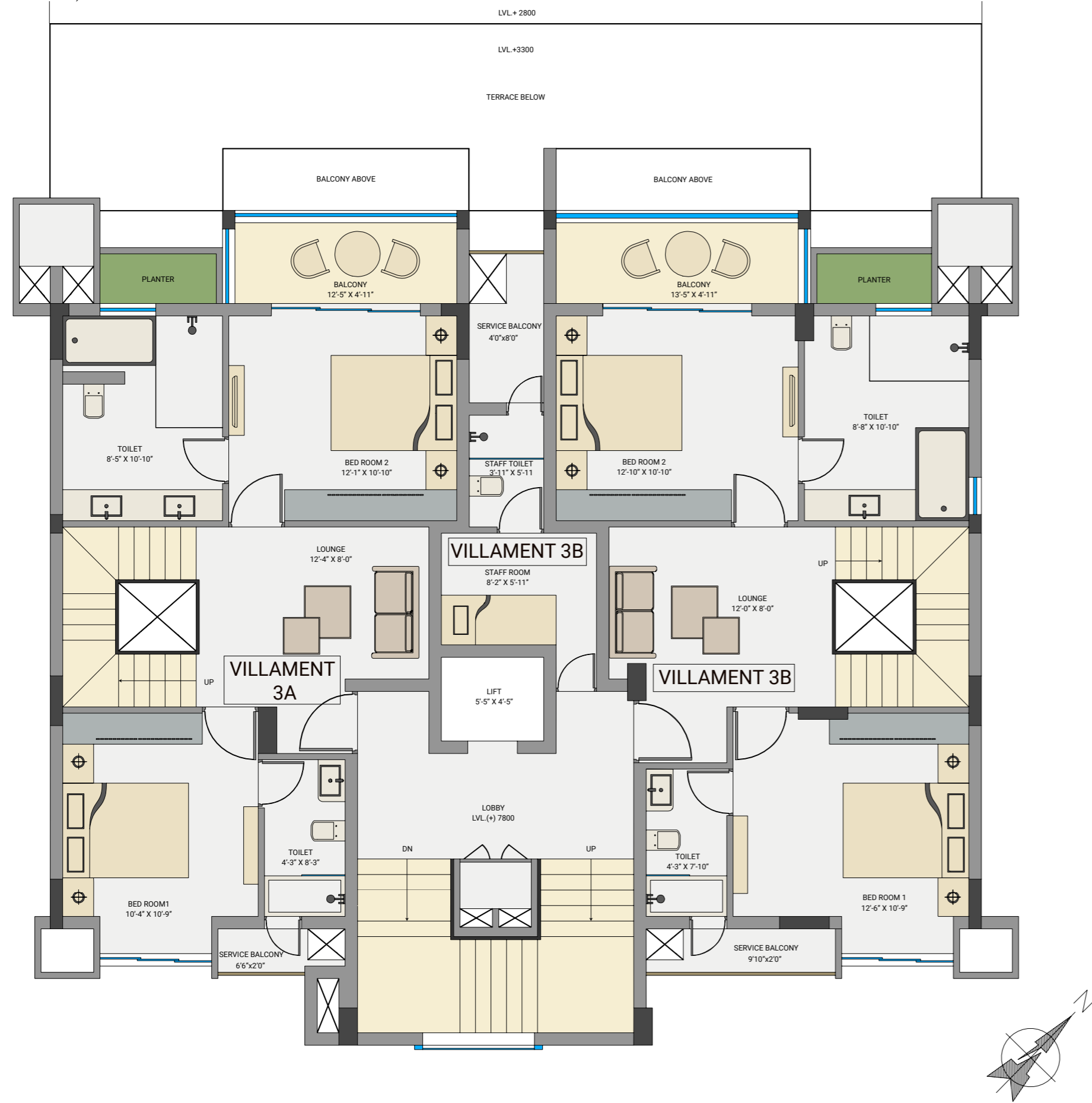
CENTER VILLAMENT 3A & VILLAMENT 3B - 2ND FLOOR PLAN (LOWER LEVEL PLAN)
