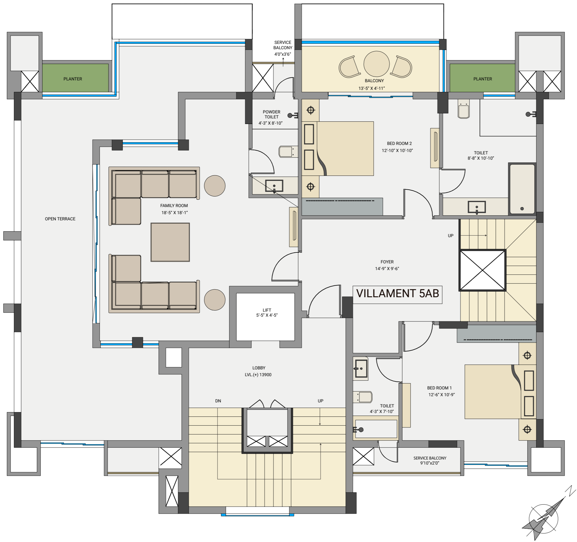
LEFT SIDE CORNER VILLAMENT 5AB - 4TH FLOOR PLAN (LOWER LEVEL PLAN)
