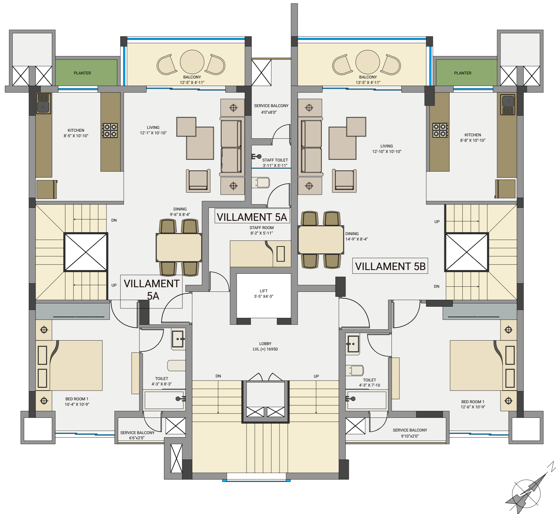
CENTER VILLAMENT 5A & VILLAMENT 5B - 5TH FLOOR PLAN (UPPER LEVEL PLAN)
